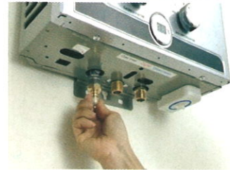
3. Open three protective covers separately.
